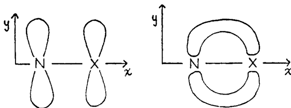
FIG. 5. Formation of a localized \pi bond
